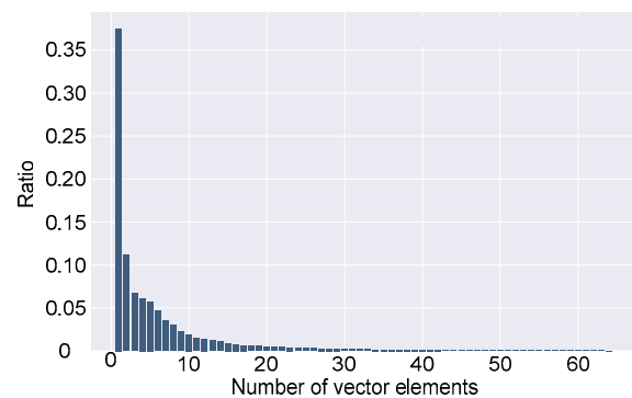
Fig. 3 Element explained variance after PCA mapping
